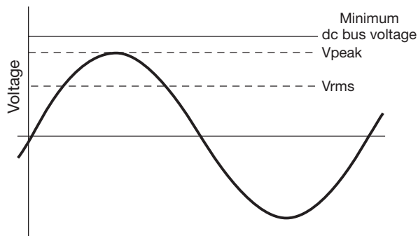
Diagram 5 The inverter's dc bus voltage must be higher than the peak ac voltage on the primary side of the transformer to create ac power from dc.
